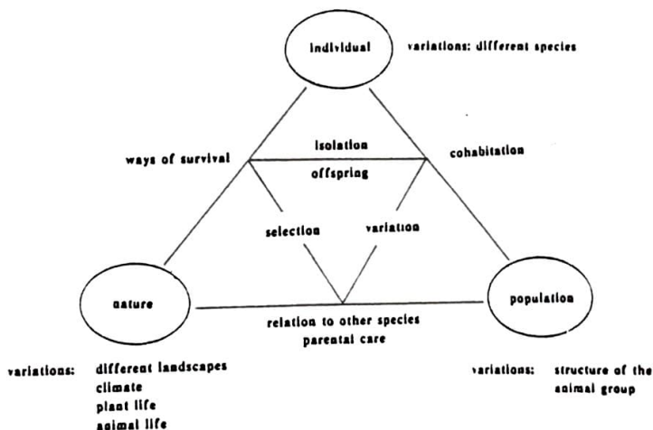
Figure 15.2. The three stages of the development of the germ-cell model (these stages are also present in the teaching process)
